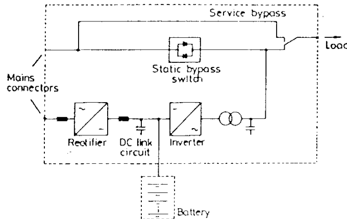
Fig 1 On line UPS Block diagram
